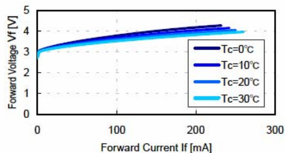
◆ Forward Voltage V f vs. Forward Current
