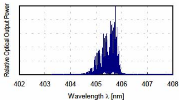
◆ Typical Spectrum
